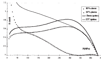
Fig. 4: Possible decomposition of grain burning surfaces of ETC ignition vs. pressure.
